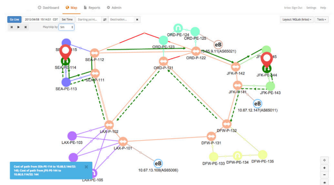
Figure 5. Example network with core routers using ICMP ECHO for hop-by-hop latency. End-to-end jitter/latency metrics are provided by full mesh shadow router connections in the regional PoPs.
