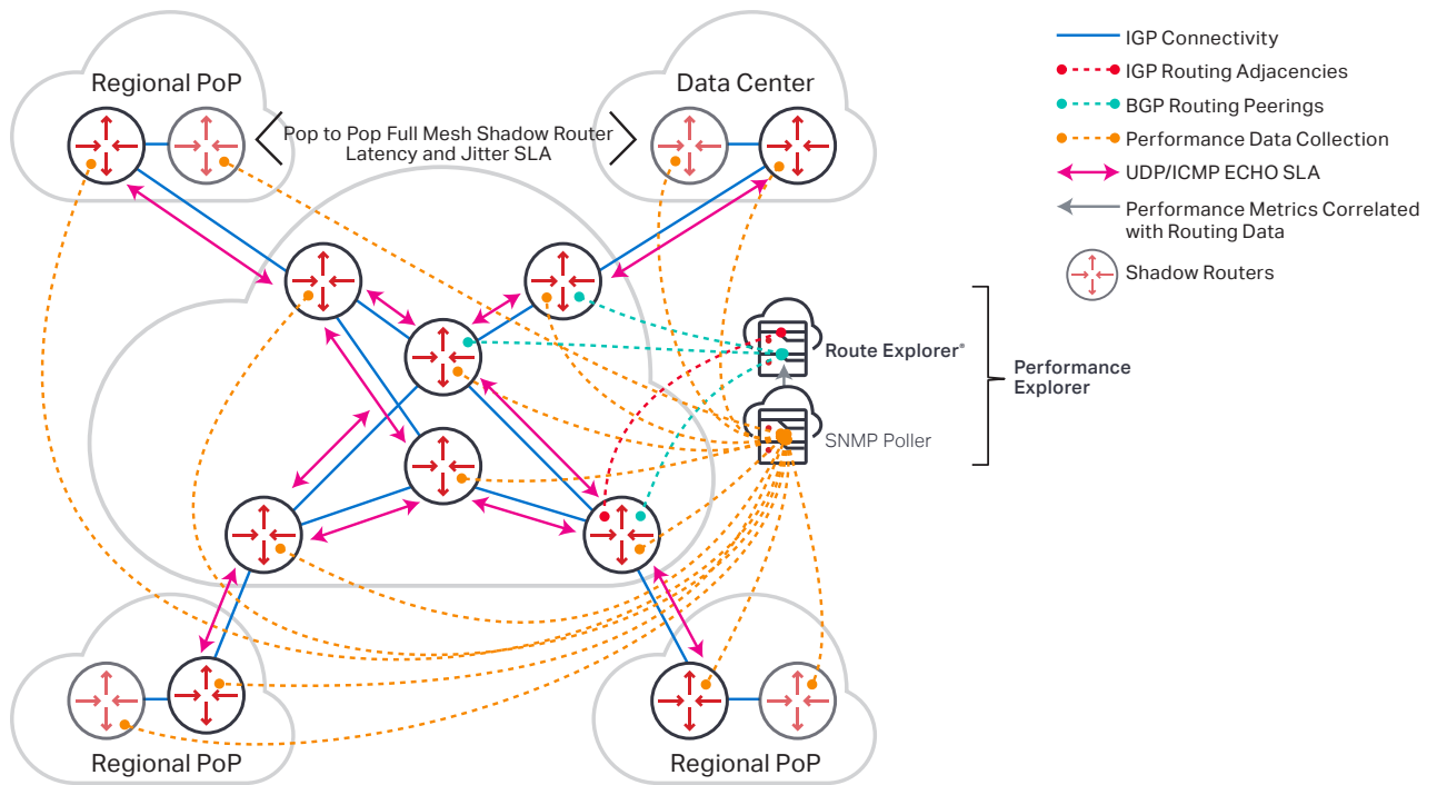
Figure 2. Performance Explorer adds SNMP metrics to Route Explorer for path-aware performance analytics.
